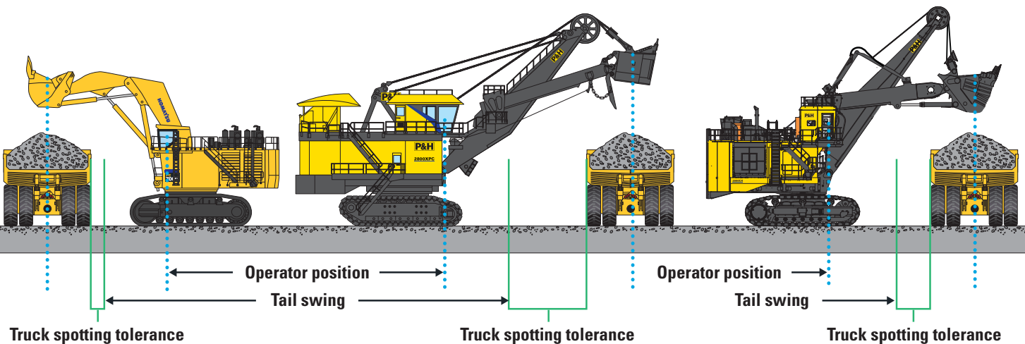
Figure 1 Truck spotting
