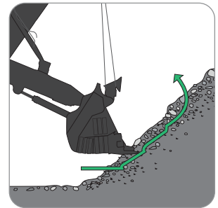
Hybrid shovel
